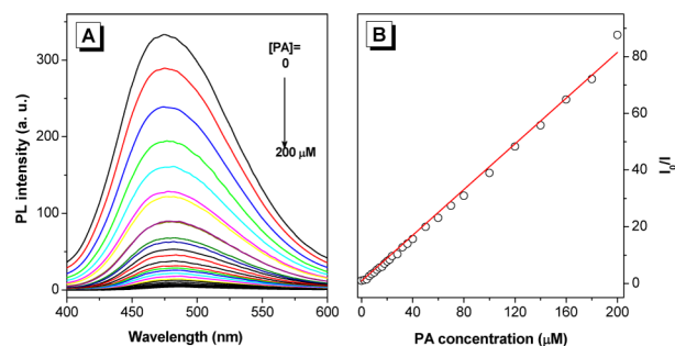
Figure 4. (A) PL spectra of PCL-TPE nanosheets suspension containing various amount of picric acid (PA) and (B) plots of I_0/I values vs PA concentrations in PCL-TPE suspension. The static quenching constant ( K ) was 380000 \text{ L mol}^{-1} for PCL-TPE nanosheets.
